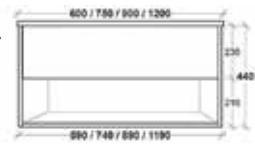
Single Drawer Wall Hung
