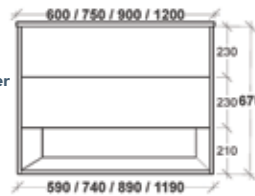
Double Drawer Wall Hung
