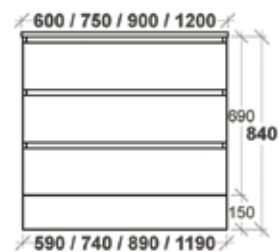
Triple Drawer Kick
