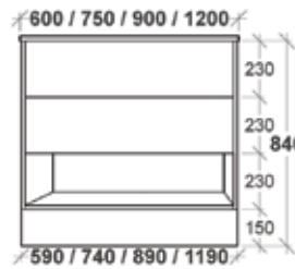
Triple Drawer Kick
